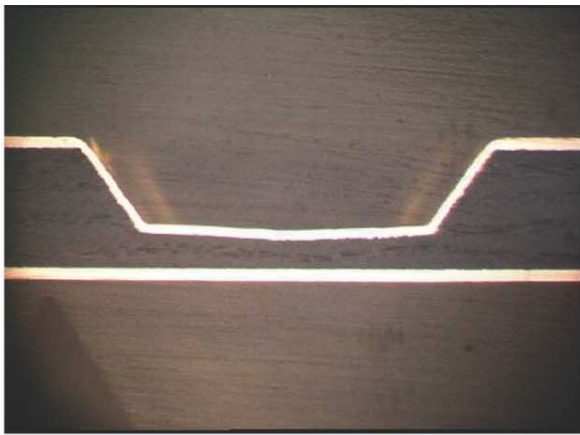
Cross-sectional image of blind via hole
